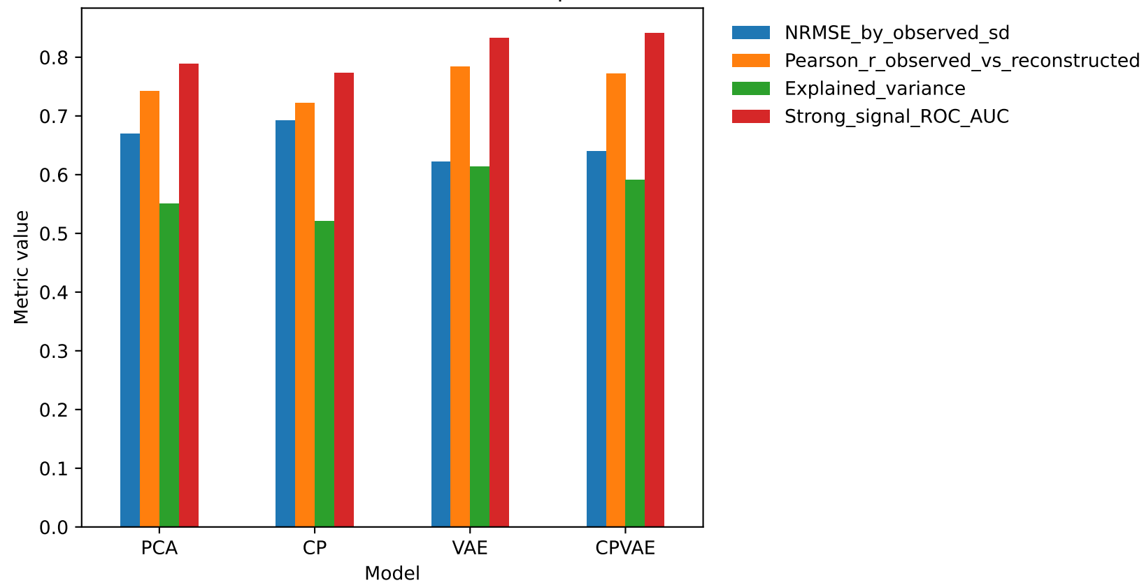
Four-model rank-6 standardized comparison
